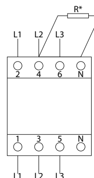
RCD ETI Type B in 3-phase system without neutral conductor - U_n=415V 30mA: R=2k\Omega/1W (500V) 300mA: R=470\Omega/2W (500V)
